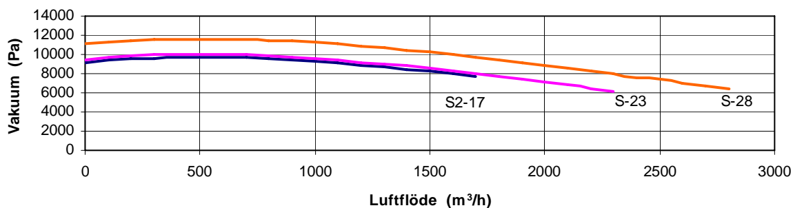
Kapacitetsdiagram S2-17, S2-23, S2-28
